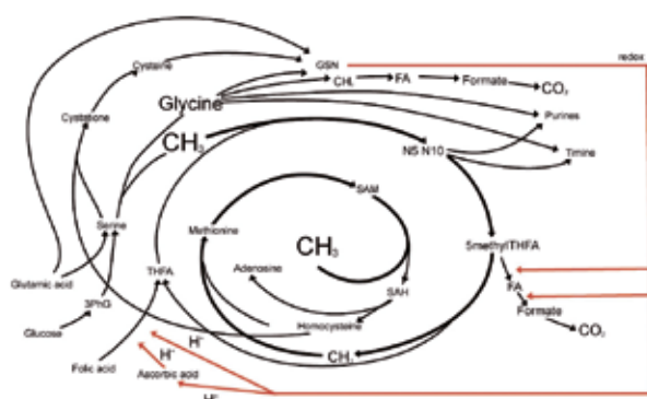
Fig. 2. In biosystem evolution there takes place a transition from unicarbon to two-carbon compounds (acetate synthesis). Formation of the reductive tricarboxylic acid cycle. Divergence of formic aldehyde and carbon dioxide ways of utilization.
