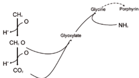
Fig. 2. In biosystem evolution there takes place a transition from unicarbon to two-carbon compounds (acetate synthesis). Formation of the reductive tricarboxylic acid cycle. Divergence of formic aldehyde and carbon dioxide ways of utilization.
